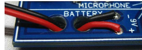
Attaching 9V Battery Snap
