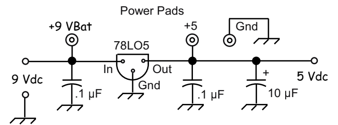
Attaching 9V Battery Snap
